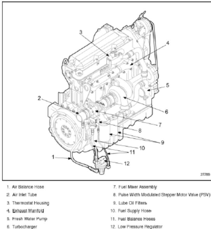
Figure 2-148 Low Pressure Fuel System (Series 60G Engine)
